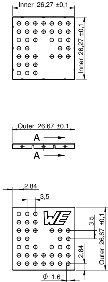
sectional drawing A-A
